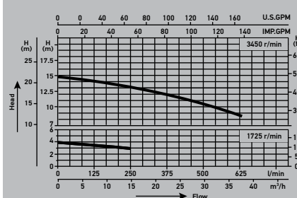
Performance curves
