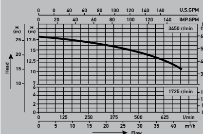
Performance curves
