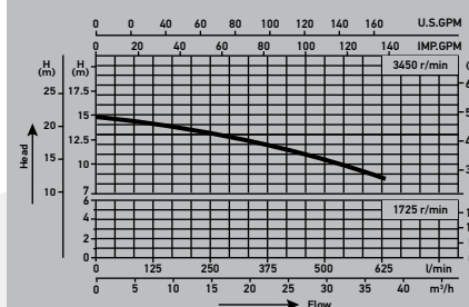
Performance curves
